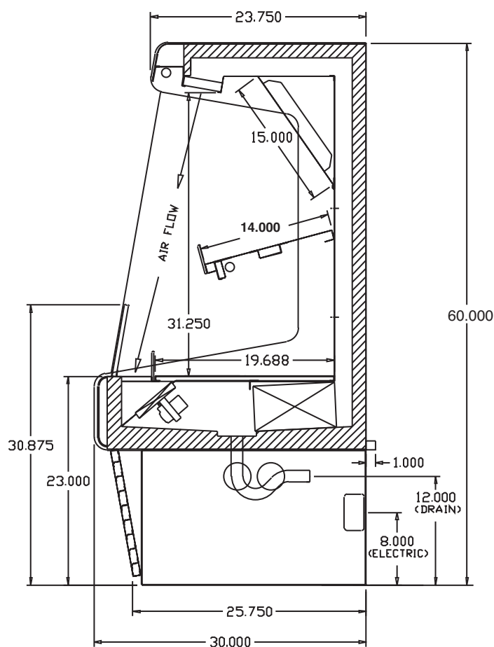
Cross Section
